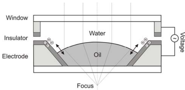
Figure 3: schematic of a tuneable lens using the electrowetting effect. With varying the applied voltage the contact angle on the inclined boundary is influenced. This is the working principle of commercially available tuneable micro lenses made by varioptic.
