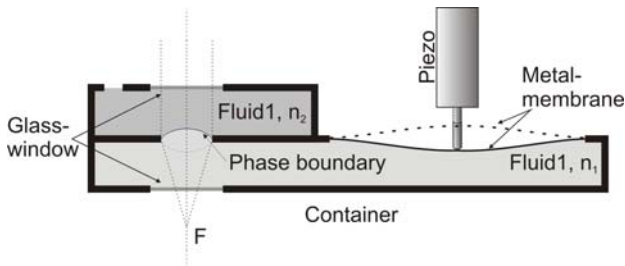
Figure 4: schematic of a tuneable lens using the piezoelectric and mechanical deformation effect combined with high frequency actuation. By applying a pressure generated by a stack of piezo actuators the a metal membrane is deformed and this deformation is transported to a immiscible liquid-liquid phase boundary to vary the focal length of a so produced liquid lens.
