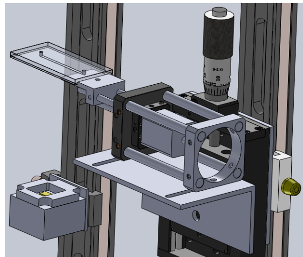
Figure 5: sketch of the experimental setup. The ferrofluid inside the micro channel follows the movement of a permanent magnet attached on a rod of a linear motor. Due to this volume so caused displacement the liquid lens is developed and can be used to focus an object on a CCD element.
